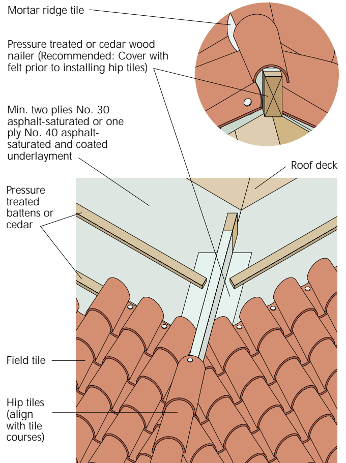
FIGURE 6C
